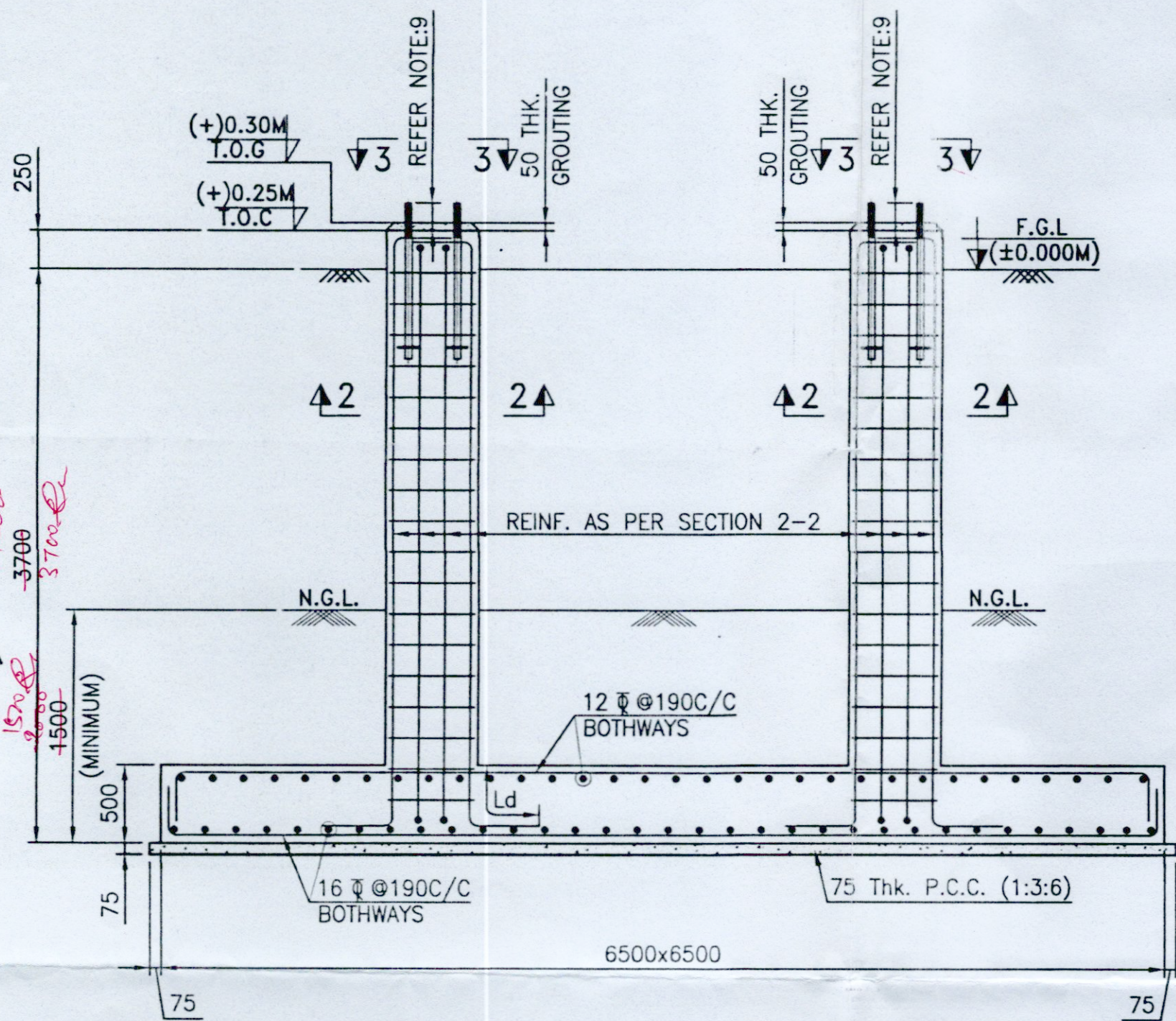
SECTION 1-1 (SCALE 1:50)
