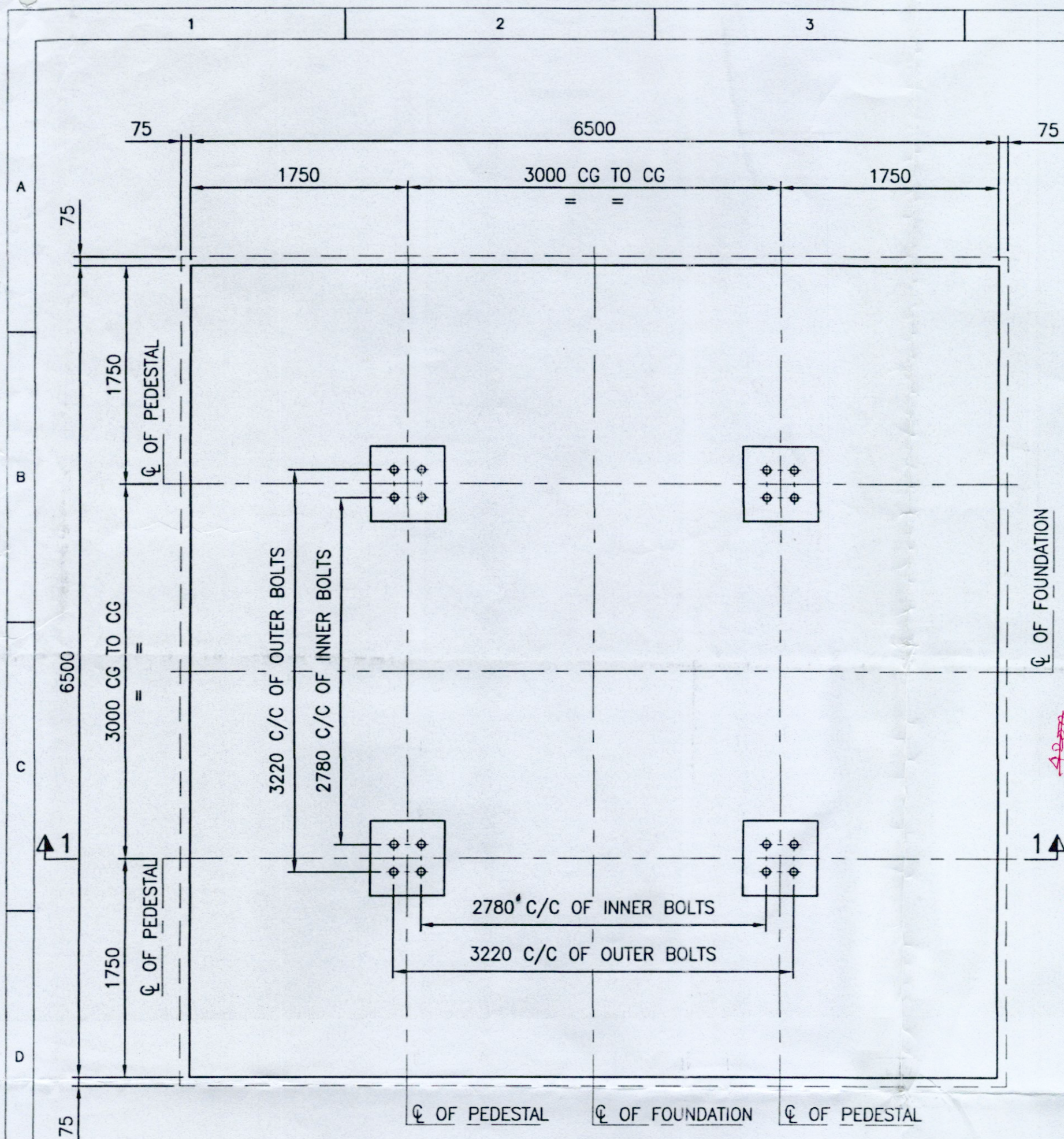
FOUNDATION PLAN (SCALE 1:50)
