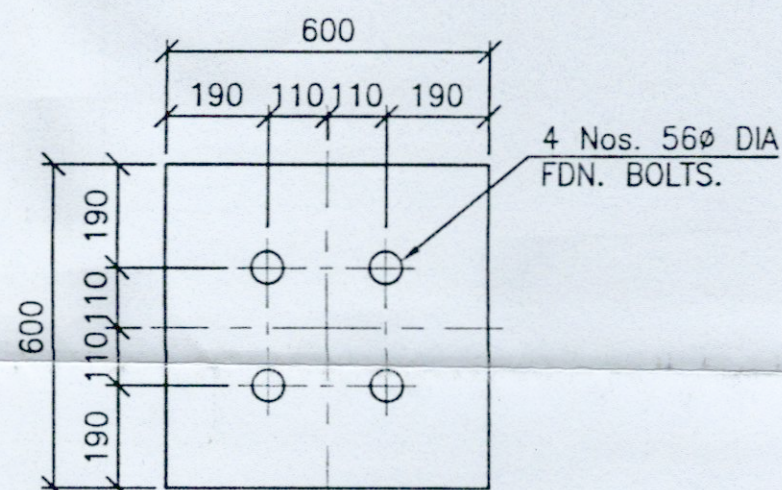
VIEW 3-3 (SCALE 1:20)
