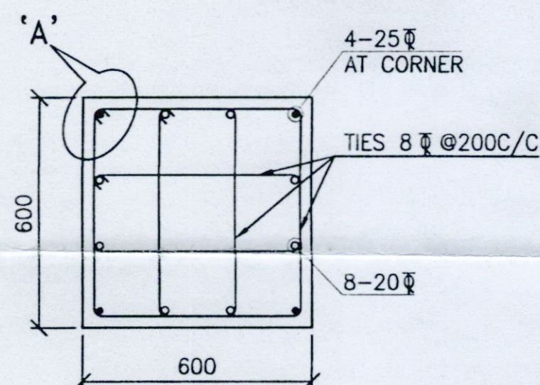
SECTION 2-2 (SCALE 1:20)
